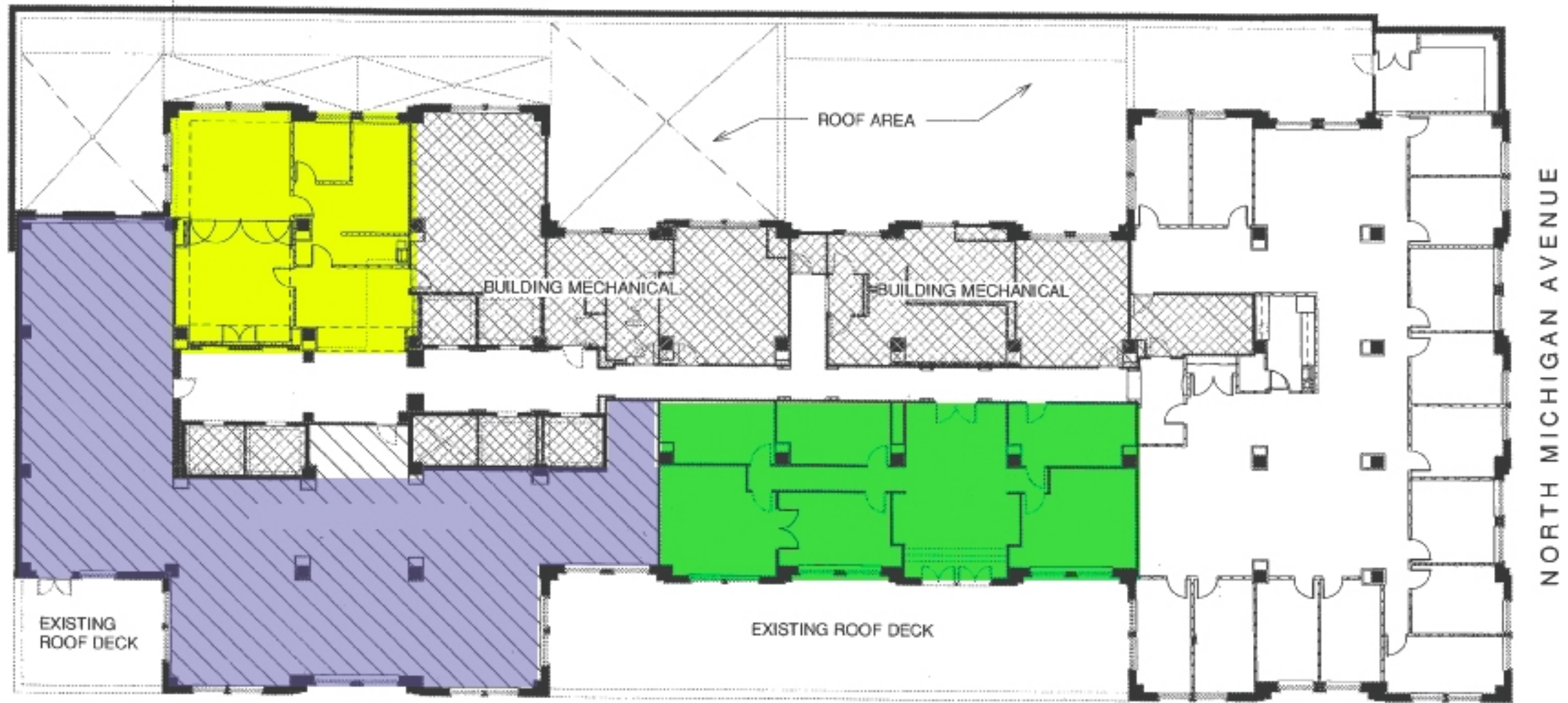
① Third Floor Key Plan 1" = 20'-0"
